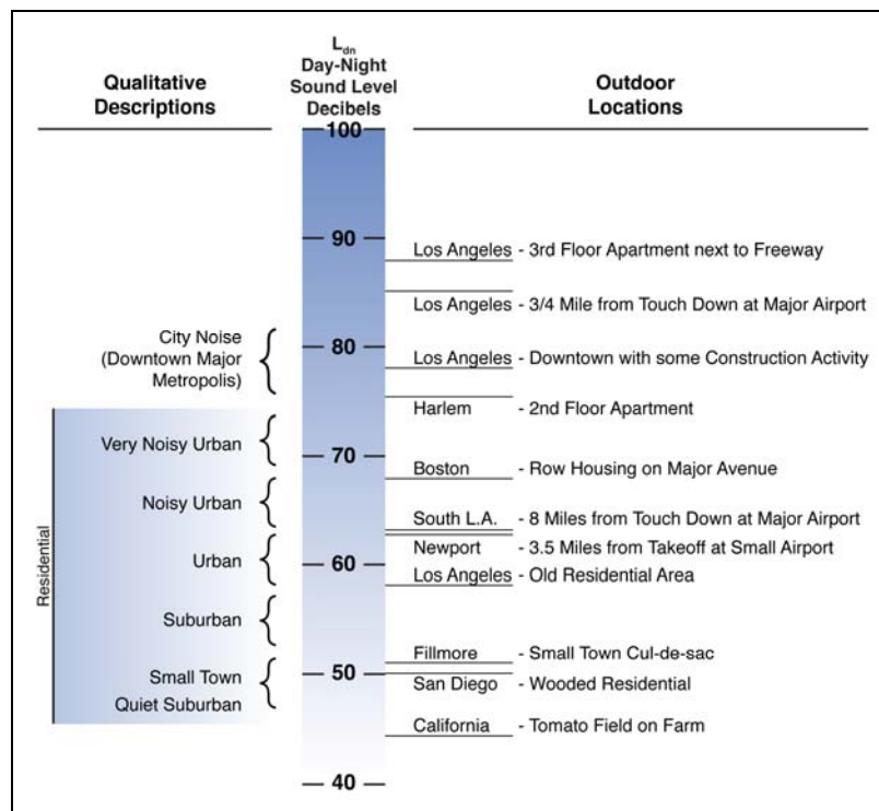
Figure C-9 Examples of Measured Day-Night Average Sound Levels
