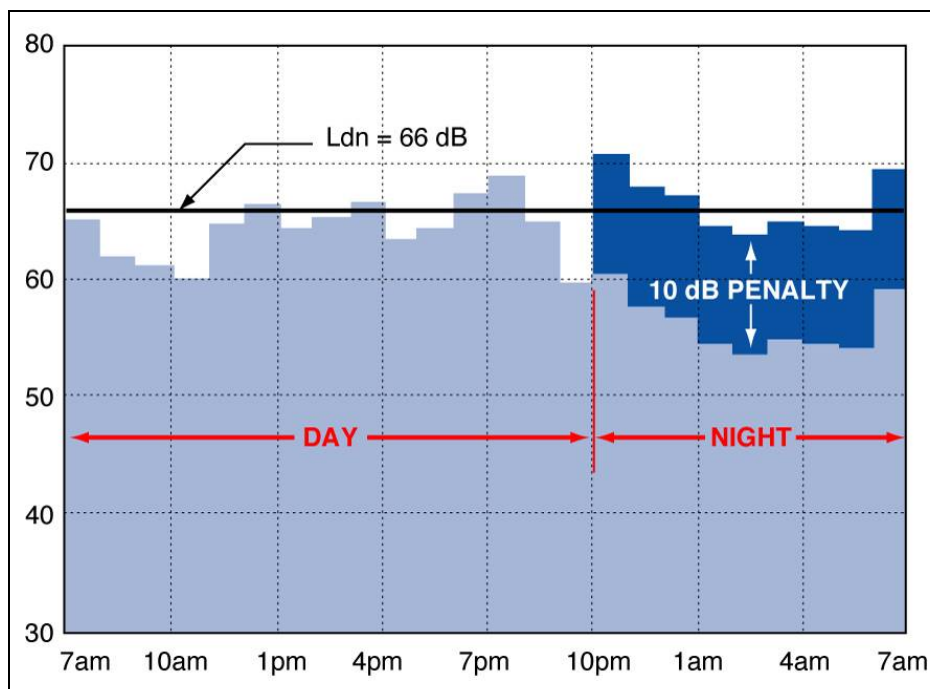
Figure C-8 Example of a Day-Night Average Sound Level Calculation
