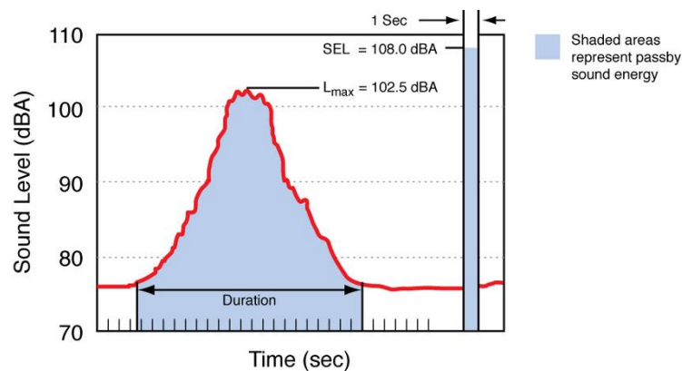
Figure C-4 Graphical Depiction of Sound Exposure Level Source: HMMH, 2011
