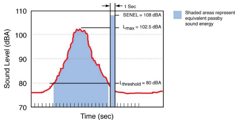
Figure C-5 Graphical Depiction of Single Event Noise Exposure Level Source: HMMH, 2011
