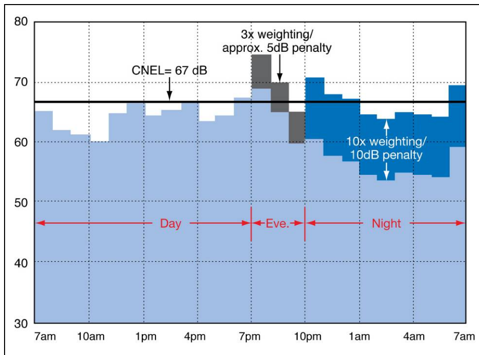
Figure C-10 Example of a Community Noise Equivalent Level Calculation
