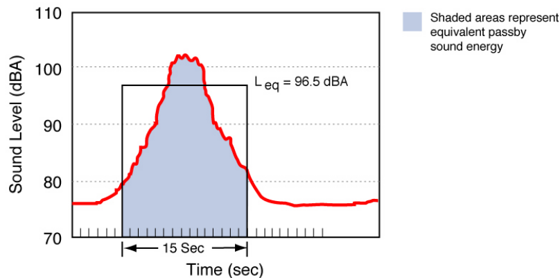
Figure C-7 Example of a One-Minute Equivalent Sound Level
